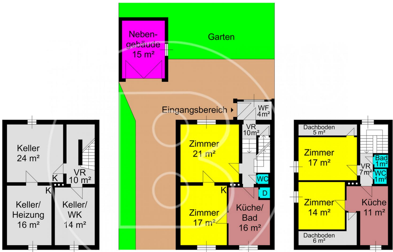
K ... Kamin D ... Dusche VR ... Vorraum WF ... Windfang Skizze Erdgeschoss
